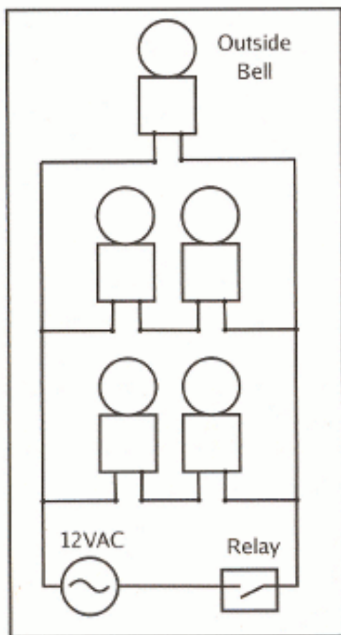
Figure 1. Schematic of the Bell System
