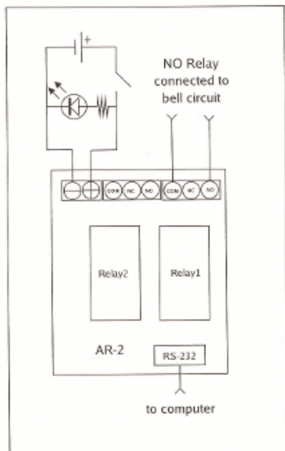
Figure 2. Connections to the AR-2 Board
